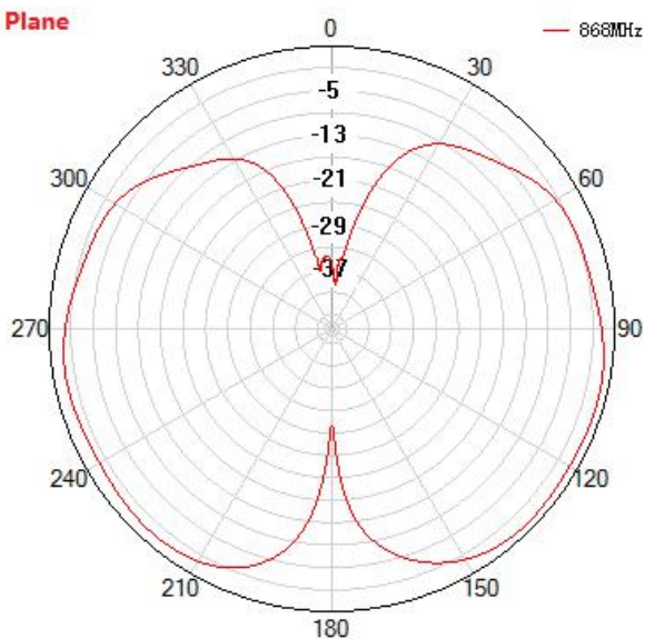
— 868MHz V Plane
